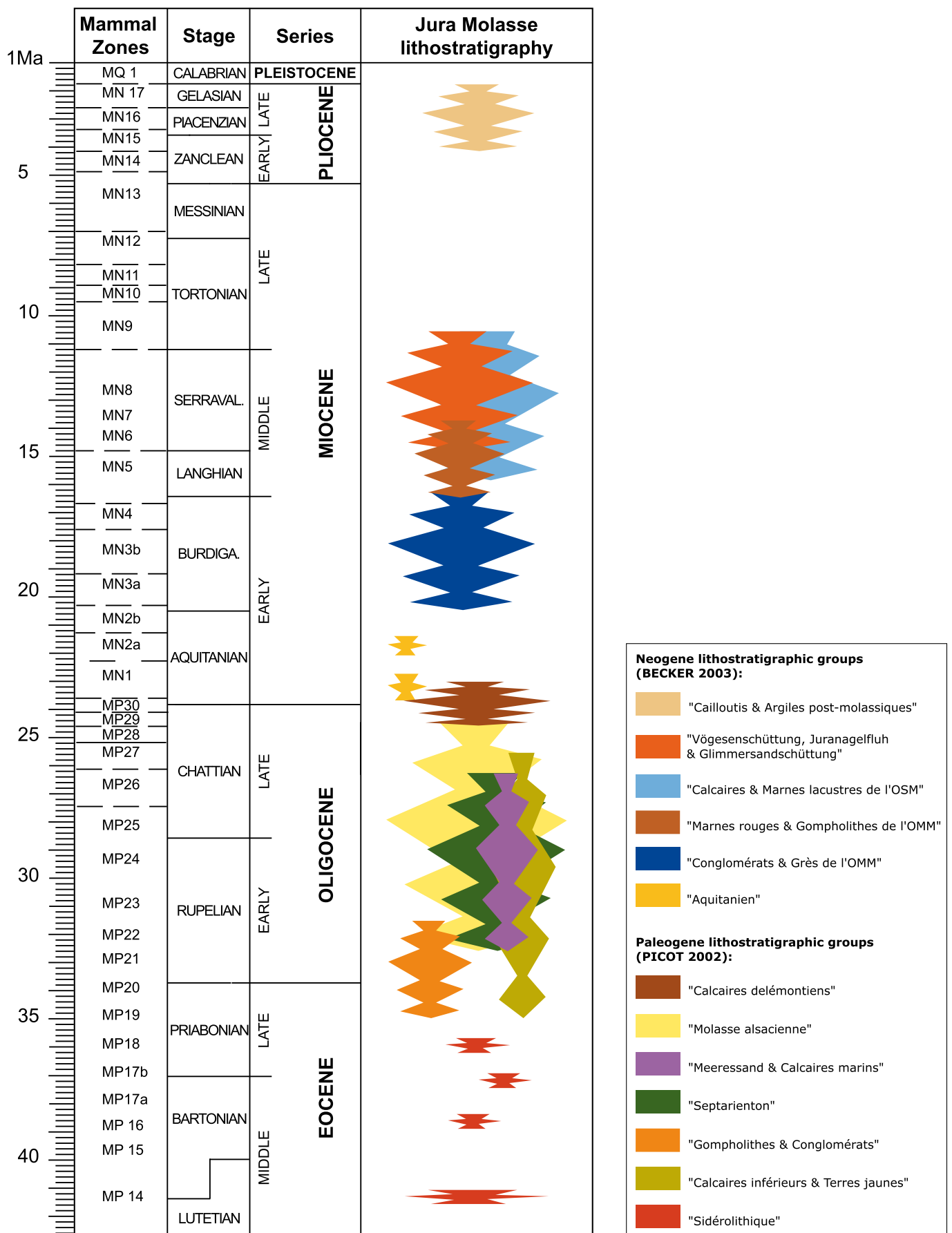
Fig. 5: Biostratigraphy and lithostratigraphy of the Jura Molasse (modified from Picot 2002 and Becker 2003).
