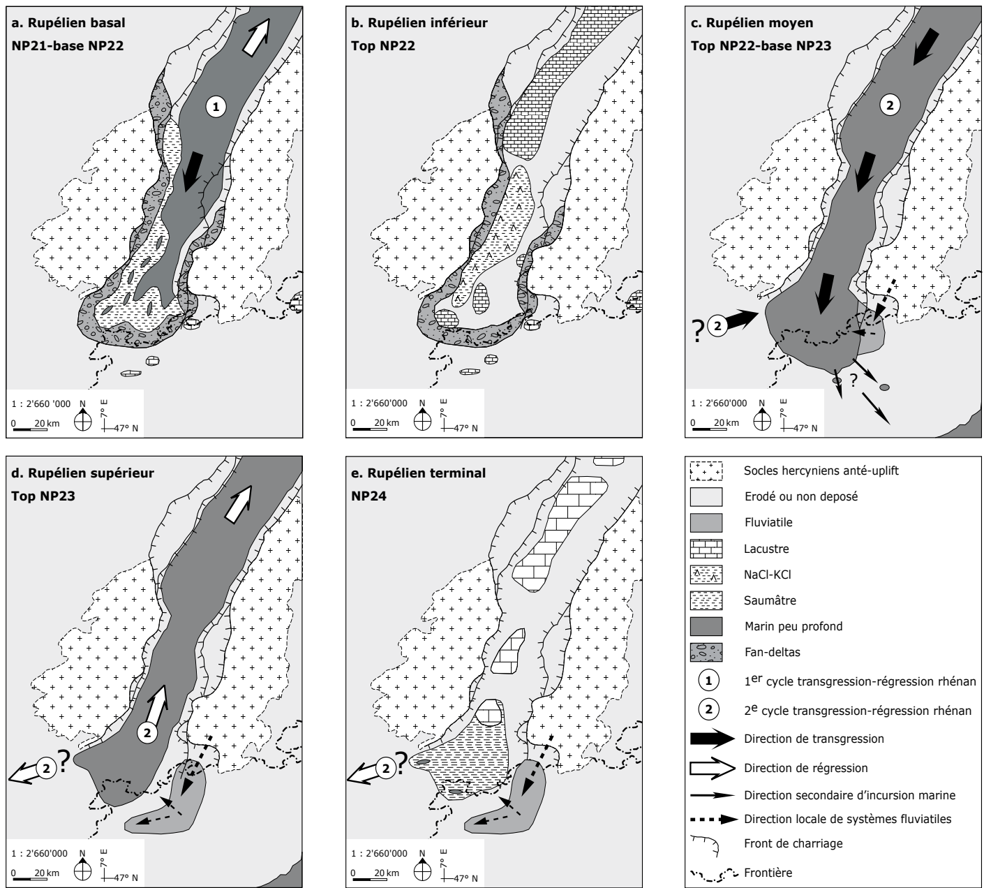
Fig. 8 : Paleogeographical evolution of the rhinish UMM in southern Rhine Graben and northern Jura.
